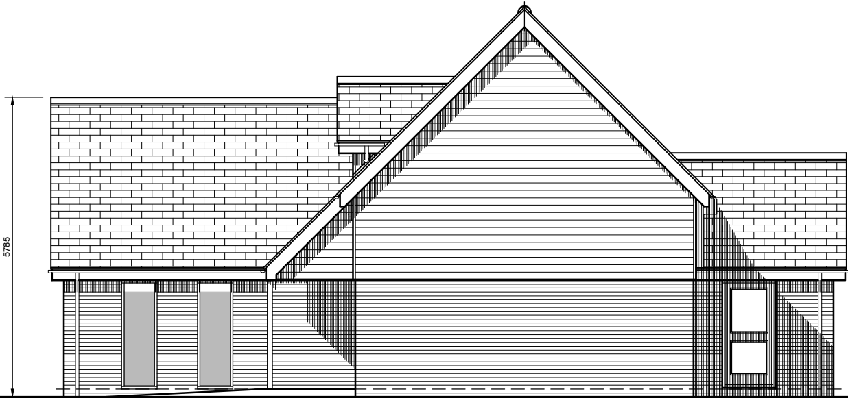
South Elevation
